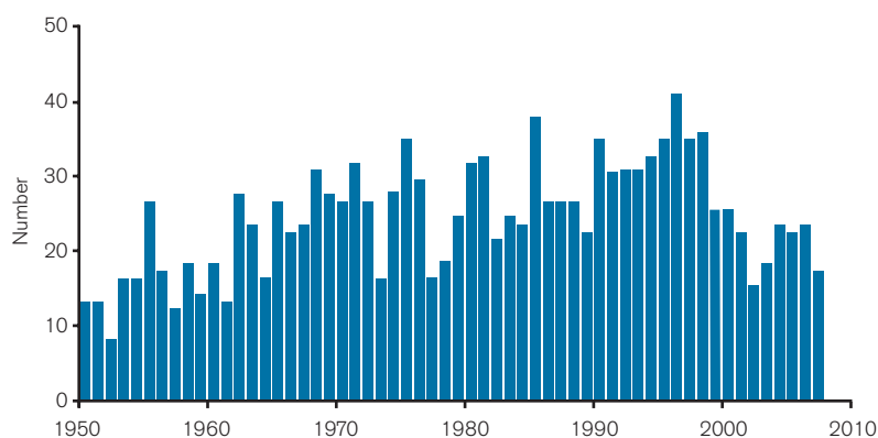
Figure 3.10: Major discoveries of non-ferrous metals (1950–2008)
